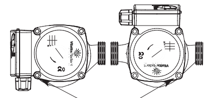
Remove allen screws to rotate pump head. Should only be done if necessary to fit an enclosure.
