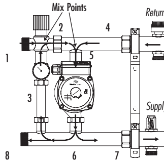
Remove allen screws to rotate pump head. Should only be done if necessary to fit an enclosure.
