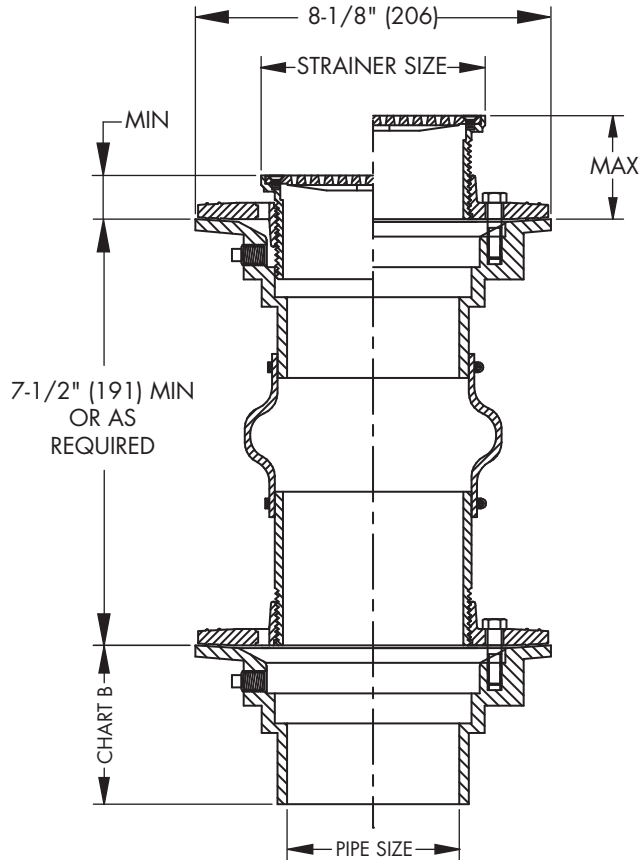
Strainer Size
