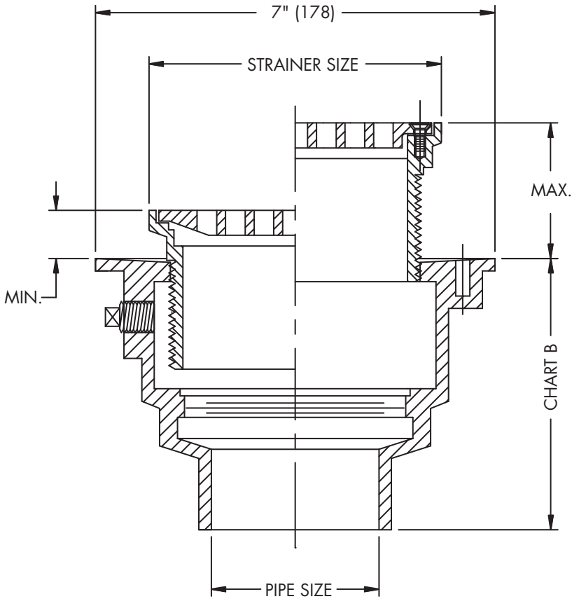
Strainer Size
