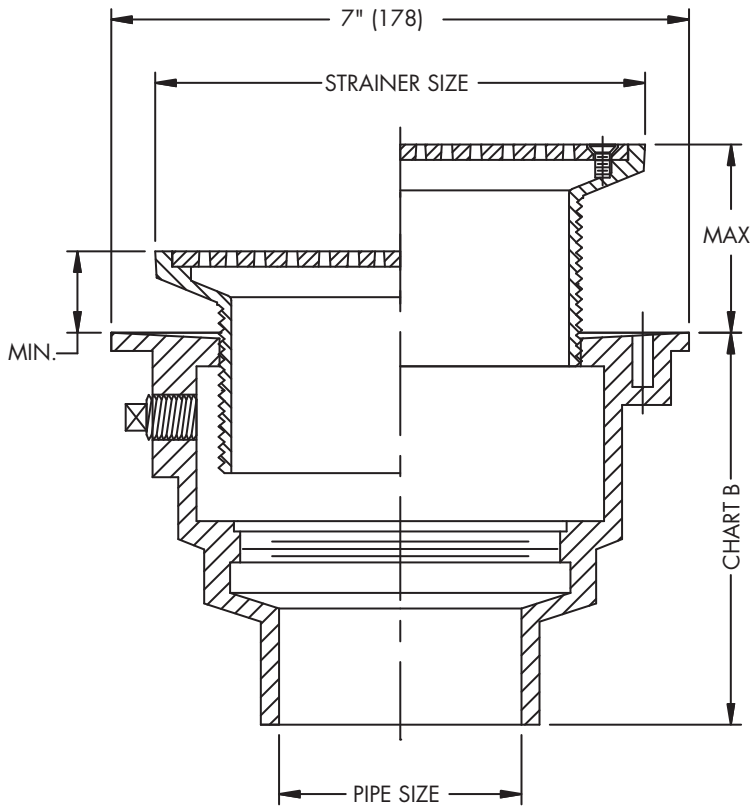
Strainer Size
