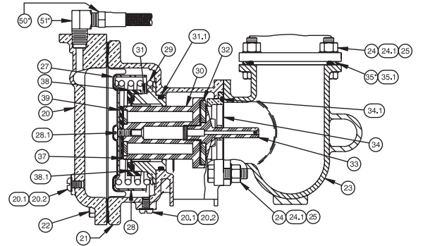
Relief Valve Detail
