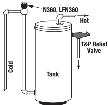
Domestic Hot Water Supply Tanks and Heaters with Bottom Feed
