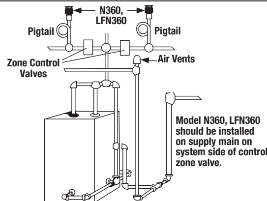
Low Pressure Steam Heating Systems
