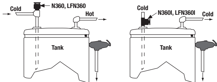
Domestic Hot Water Supply Tanks and Heaters with Top Supply
